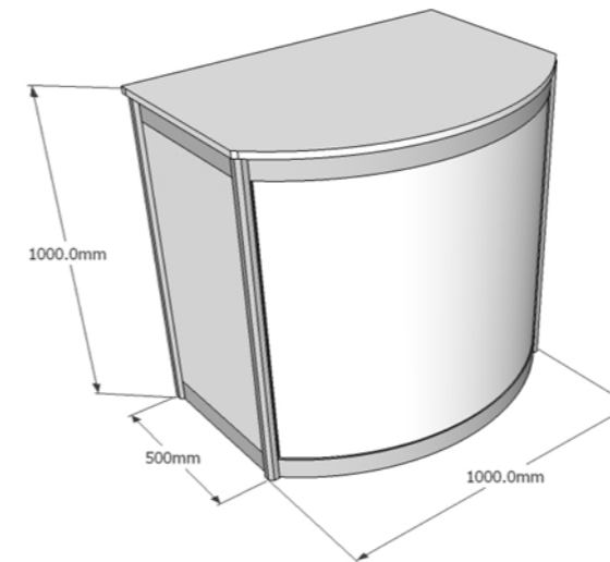
Counter #7 As per counter #4 with curved front
