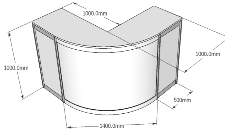
Counter #6 Includes internal shelf plus lockable doors (2)
