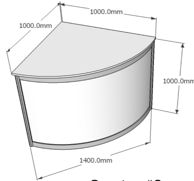
Counter #3 Quarter Circle Lockable door to rear Excludes internal shelf
