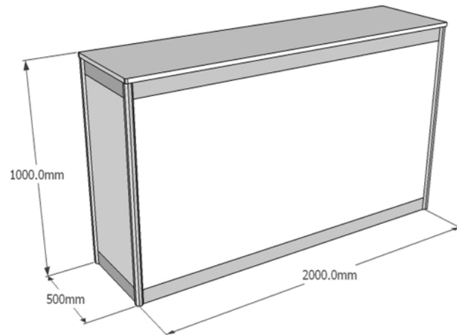
Counter #5 Includes internal shelf plus lockable doors to rear
