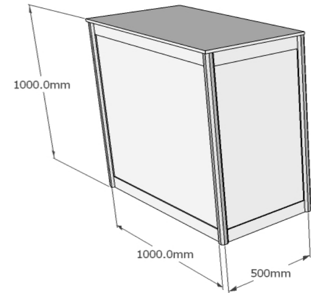
Counter #4 Includes internal shelf plus lockable doors
