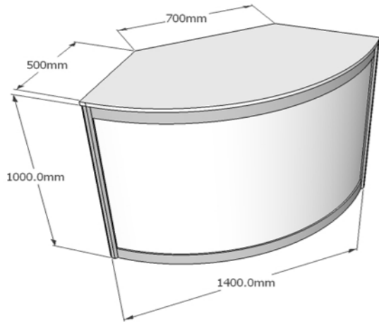
Counter #1 Includes lockable door to rear plus internal shelf
